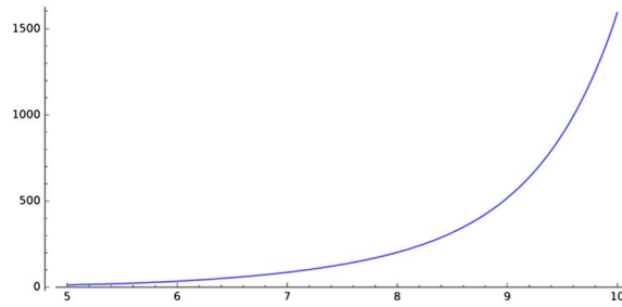
Fig. 4. \tilde{G}_{1/5}(x) .
