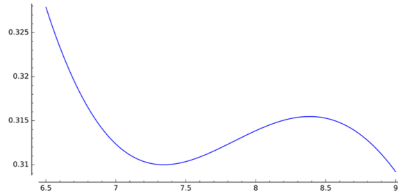
Fig. 3. x^{-1}G_{1/5}(x^{-5}) .
