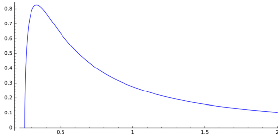
Fig. 1. The free positive 1/2-stable density (WS).
