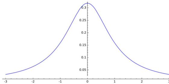
Fig. 2. The free symmetric 1-stable density (BS).
