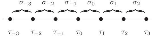
Fig. 1. Delaunay decomposition
