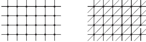
Fig. 4. Delaunay decompositions
