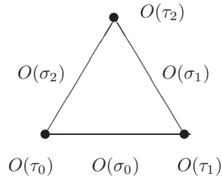
Fig. 2. A 3-gon
