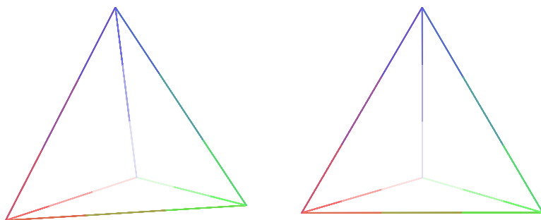
Figure 1: 正四面体
