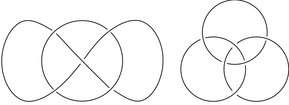
Figure 1: the Whitehead link and the Borromean rings
