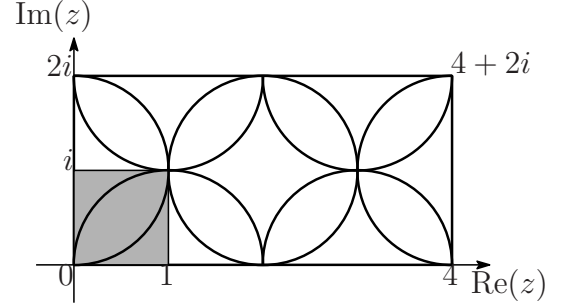
Figure 3: Fundamental domain of G_B in \mathbb{H}^3
