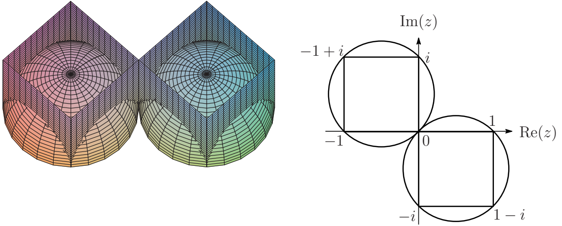
Figure 2: Fundamental domain of G_W in \mathbb{H}^3
