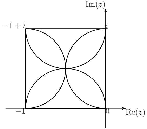
Figure 4: Weyl chamber of \Gamma^T(2)
