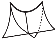
folded umbrella
