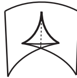
swallowtail
