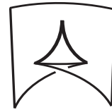
open swallowtail
