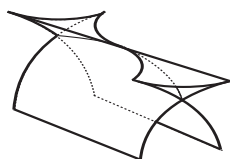
Mond surface (cuspidal-beaks)
