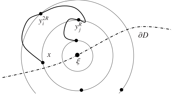
FIGURE 3. A cigar curve connecting x to \xi .
